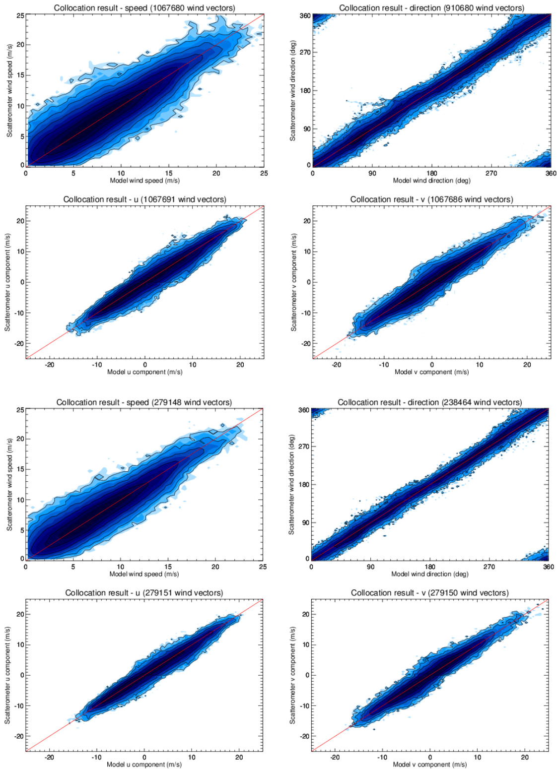
Figure 2: Two-dimensional histograms of wind speed, direction (w.r.t. wind coming from the North), u and v components of 25 km (top) and 50 km (bottom) RapidScat wind product versus the ECMWF model forecast winds from 25 and 26 January 2015.
