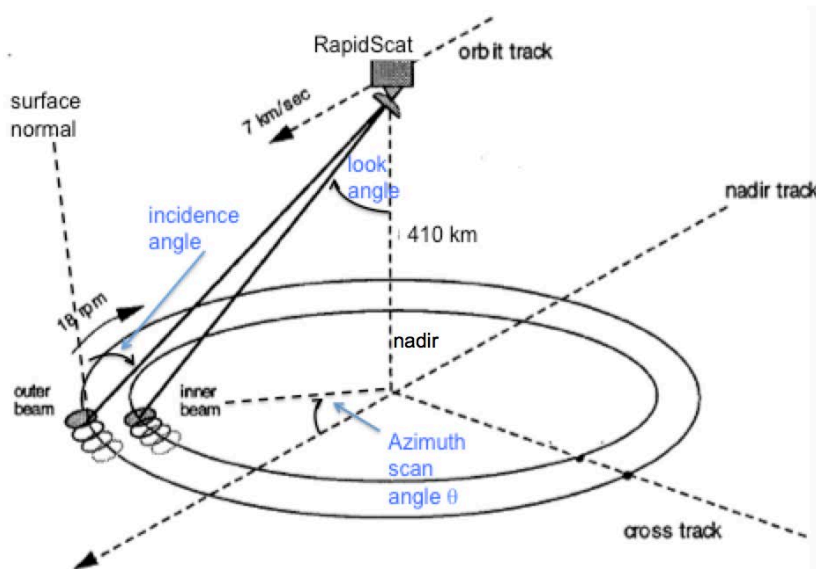
Figure 1: RapidScat pencil beam geometry (source: JPL web site).
