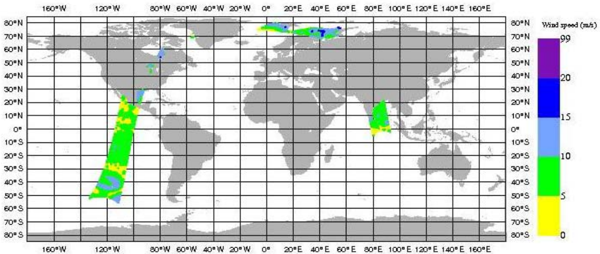
Figure 2.4 Global coverage of the testruns. Wind speed results for testrun 2 are shown.
