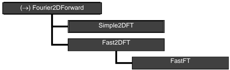
Figure B2.5 Calling tree for AR routine Fourier2DForward . The calling tree for routine Fourier2DBackward is identical.
