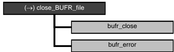
Figure B3.4 Calling tree for BUFR handling routine close_BUFR_file .
